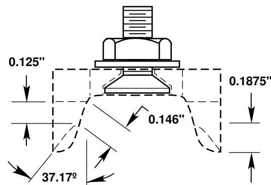
SIDE VIEW SADDLE W/HARDWARE
